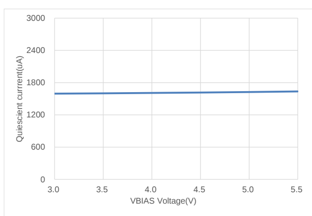
BIAS Supply Current VS V_{BIAS}
