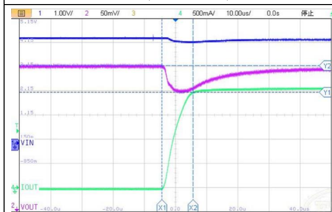
Load Transient Response V_{IN}=4.25V , V_{OUT}=3.95V , I_{OUT}=1mA\sim 2000mA
