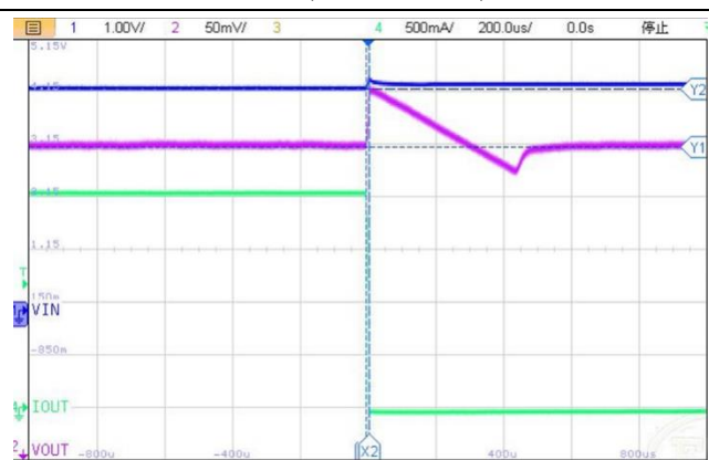
Load Transient Response V_{IN}=4.25V , V_{OUT}=3.95V , I_{OUT}=2000mA\sim 1mA
