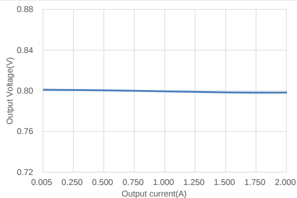
Output Voltage VS Output Current ( V_{IN}=1.4V , no V_{BIAS} )
