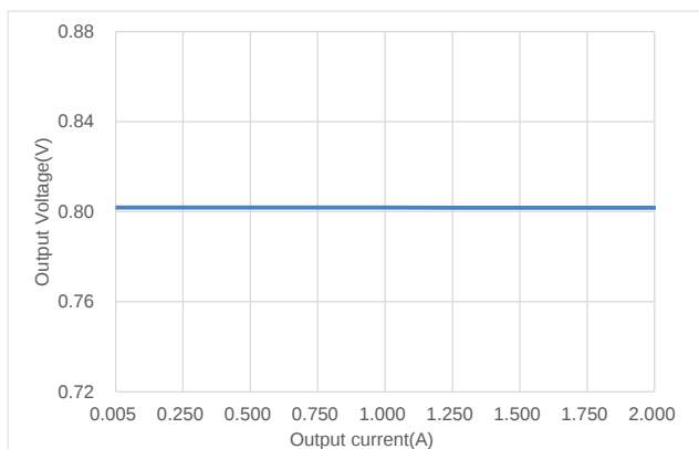
Output Voltage VS Output Current ( V_{IN}=1.1V )
