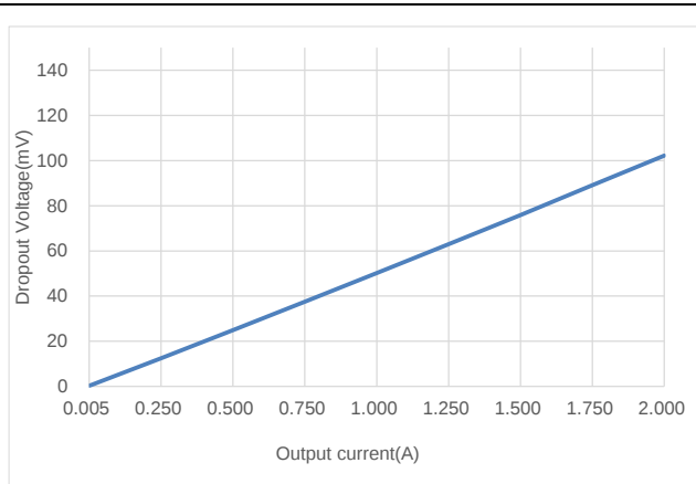
Drop Voltage VS Output Current
