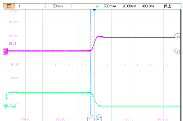
Load transient(0.5A~1mA t=10\mu s \Delta V=52.5mV )
