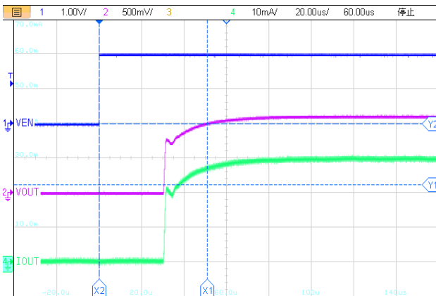
t_{ON}=51\mu\text{s} ( I_{OUT}=30\text{mA} )
