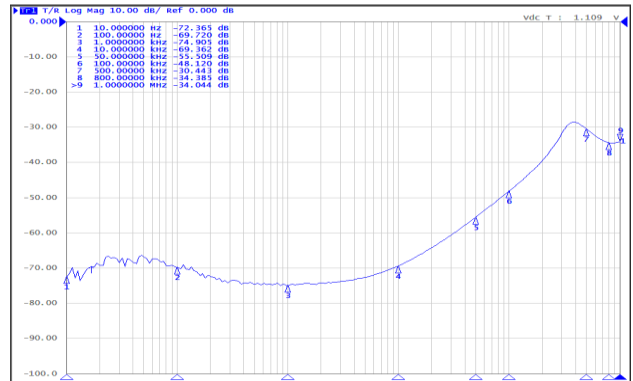
PSRR Test( I_{OUT}=0.5\text{A} )
