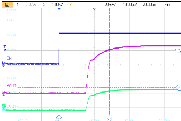
t_{ON}=28.6\mu s(I_{OUT}=30mA)
