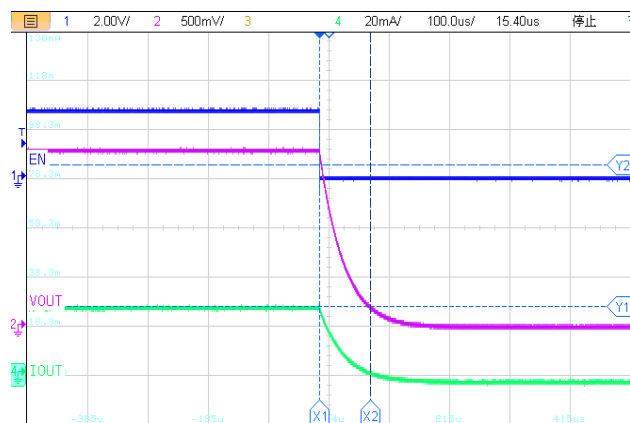
t_{OFF}=84\mu\text{s} ( I_{OUT}=30\text{mA} )
