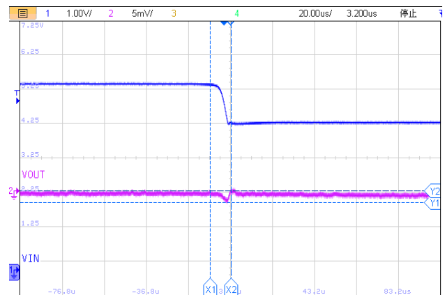
Line transient(5.5~4.3V t=10\mu s \Delta V=1.7mV )
