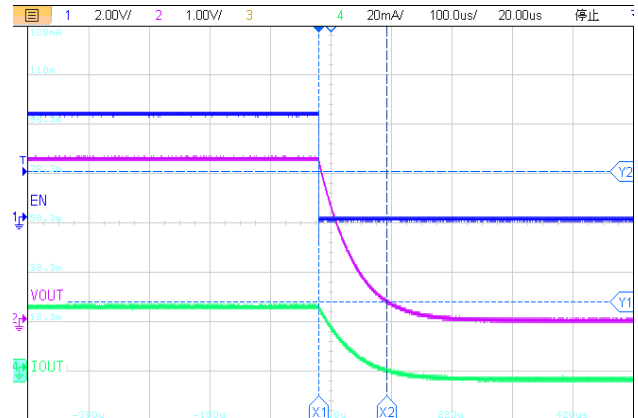
t_{OFF}=112\mu s(I_{OUT}=30mA)
