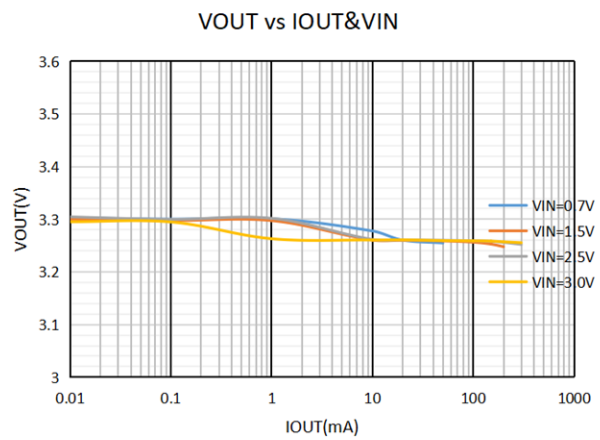
Figure2.Load Regulation
