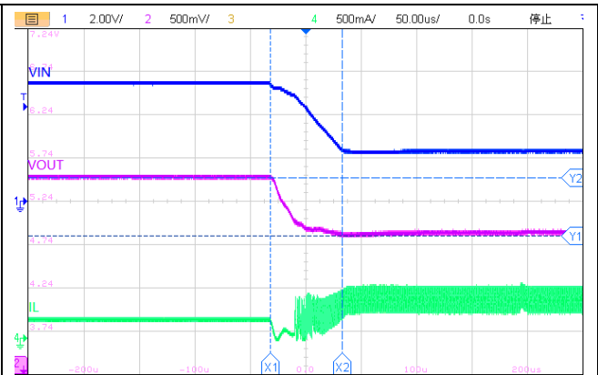
Figure18.Line Transient
