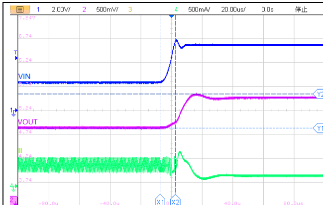
Figure17.Line Transient
