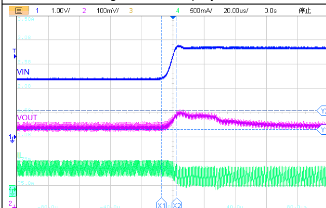
Figure13.Startup by V_{IN}
