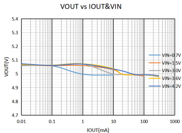
Figure2.Load Regulation
