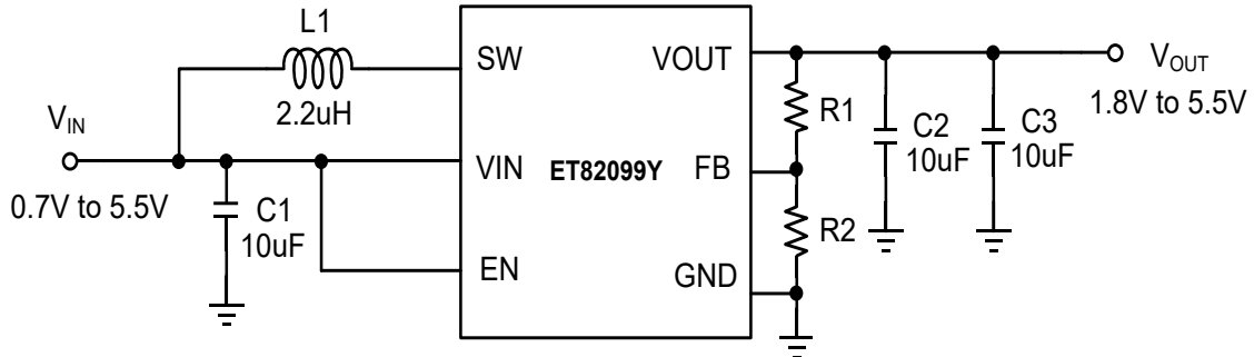
ET82099Y Application Circuit
