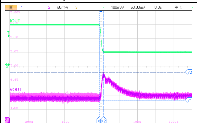
Figure20.Load Transient
