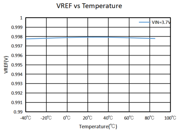
ET82099Y, V_{IN}=3.7V , T_A=-40^{\circ}C\sim 85^{\circ}C Figure 8. Reference Voltage vs Temperature
