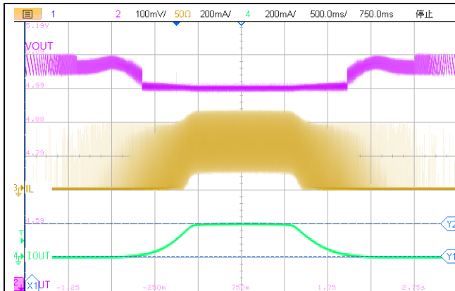
V_{IN}=3.7V, V_{OUT}=5V, I_{OUT}=0mA \text{ to } 200mA Figure23.Load Transient
