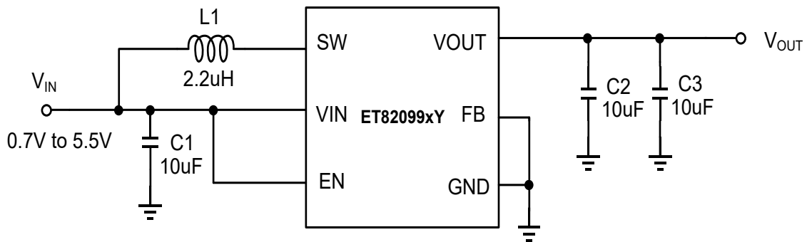
ET82099xY Application Circuit
